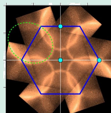
Fermi surface of the topological Kondo insulator \text{SmB}_6(111) surface obtained by an angle-resolved photoelectron spectroscopy.
