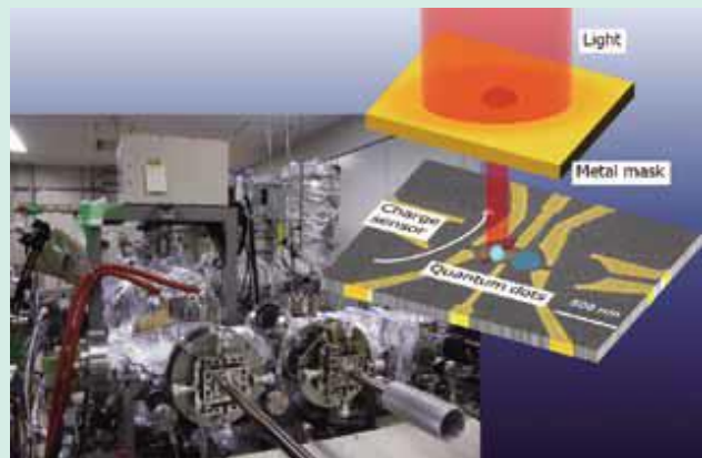
(Left) Molecular beam epitaxy, (Right) Schematic illustration of photon-spin quantum interface using a quantum dot
