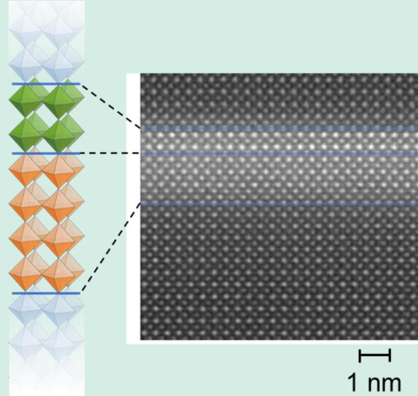
An artificial interface structure consisting of three kinds of correlated oxides
